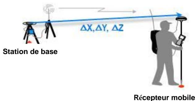
Figure 2-1 Configuration type du RTK
