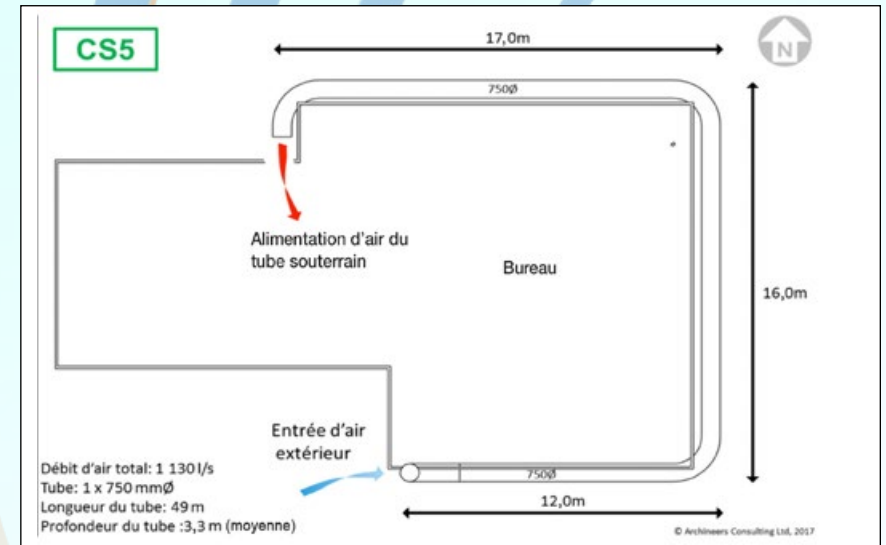
Figure 4. Configuration des tubes.
